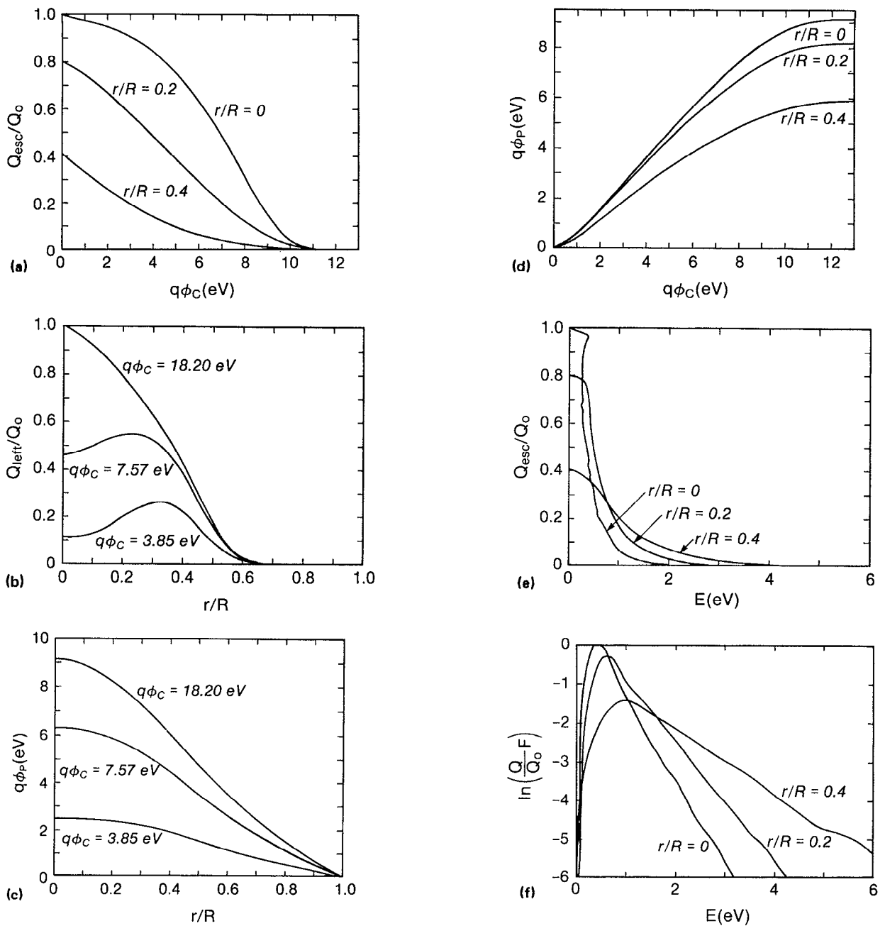
FIG. 2. Measured density data, and derived potentials and energies. (a) Measured escaping charge Q_{\text{esc}} versus applied confinement potential \phi_c at several radii. Q_{\text{esc}} is normalized to Q_0 = Q_{\text{esc}}(r=0, \phi_c=0) . (b) Remaining charge versus the normalized radius, for several confinement potentials \phi_c . (c) Plasma potential \phi_p versus radius. \phi_p is calculated from the data of (b), using Eq. (4). (d) Calculated plasma potential \phi_p versus confinement potential \phi_c . (e) Measured Q_{\text{esc}} as a function of calculated E = q(\phi_c - \phi_p) . (f) Resulting energy distribution function F(E) , normalized by Q/Q_0 .
