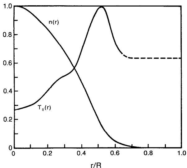
FIG. 3. Experimentally obtained density and parallel temperature profiles, normalized to their maximum values. The dashed portion of the temperature curve is unobtainable, but is specified to be flat for the parameter fit.
