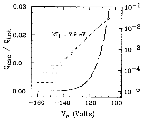
FIG. 4. Escaping charge Q_{\text{esc}}/Q_{\text{tot}} versus confinement voltage V_c on linear and logarithmic scales. Q_{\text{tot}} is the total charge initially trapped.
